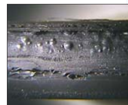
O-ring exposed to rapid depressurization
